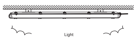
9. Buckle the clips
