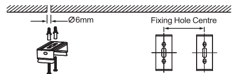
2. According to the Fixing hole centre, install expansion bolts and screws, install the bracket.
